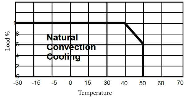
Derating curve
